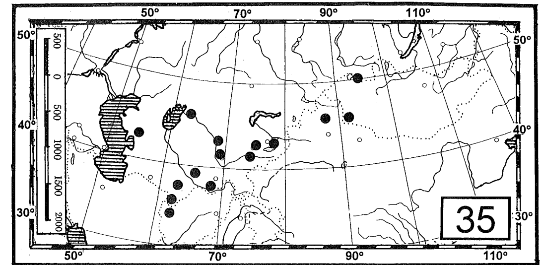
Fig. 35 - Distribution of Synageles ramitus ANDREEVA, 1976.
