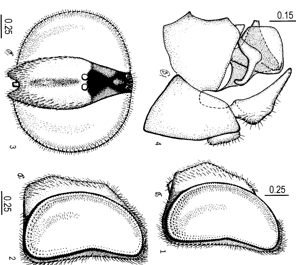
Figs 1-4: Paragus sinicus spec. nov. – 1. ♂ head, lateral; – 2. ♀ head, lateral; – 3. ♀ head, frontal; – 4. ♂ genitalia, lateral. – Scales in mm.
