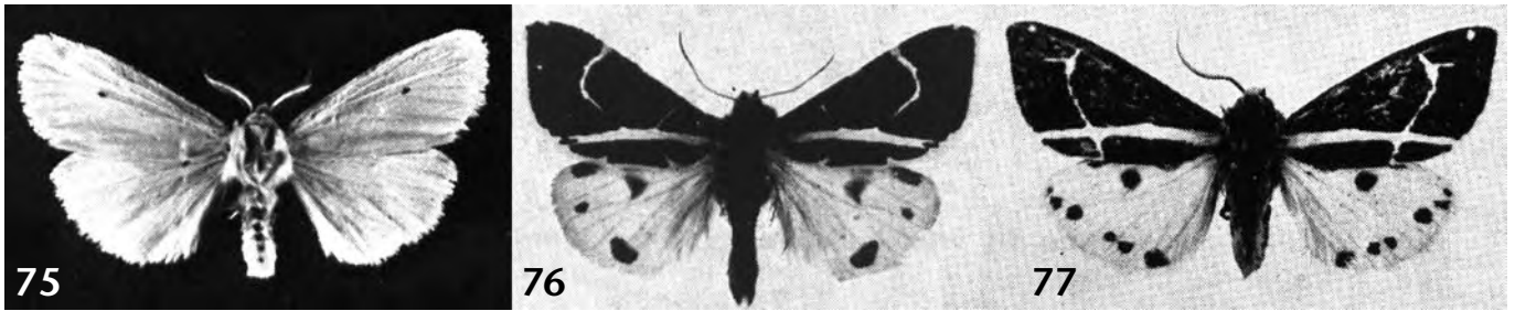
Figs. 75–77: Reproductions from DE TOULGOËT (1980, 1986). Fig. 75: Popoudina brosi , ♂, from DE TOULGOËT (1986). Figs. 76–77: Specimens of Afrojavanica kostlani (76) and A. melaena (77), from DE TOULGOËT (1980). — Not to the same scale.
